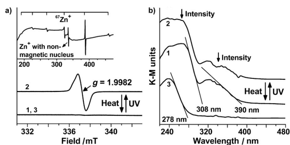
Figure 1. a) Room-temperature X-band EPR spectra and b) UV/Vis diffuse reflectance spectra of the \text{Zn}^{2+} -ZSM-5 sample in vacuum (curve 1), the (\text{Zn}^+, \text{Zn}^{2+}) -ZSM-5 sample (curve 2), and the reference \text{Zn}^{2+} -ZSM-5 sample (curve 3; K-M units = Kubelka-Munk units). The inset of Figure 1a is the EPR spectrum of the ^{67}(\text{Zn}^+, \text{Zn}^{2+}) -ZSM-5 sample. The EPR spectrum for the reference \text{Zn}^{2+} -ZSM-5 material (curve 3) is identical to that for \text{Zn}^{2+} -ZSM-5 (curve 1).
